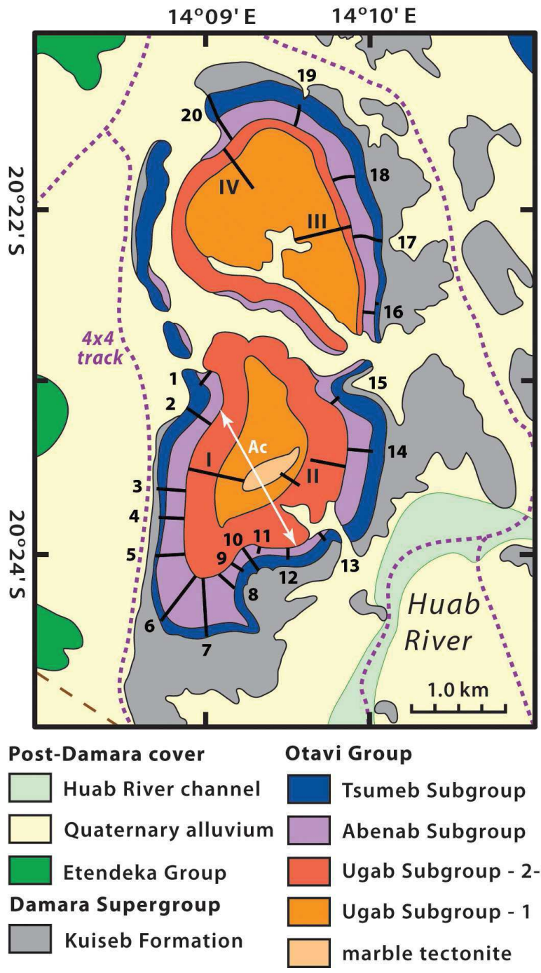
Figure 3: Geology of the Vrede domes (modified after Maloof, 2000) showing locations of measured sections of the Ugab Subgroup (sections I-IV, Fig. 5), and the Abenab Subgroup and lower Karibib Formation (sections 1-20, Fig. 6). The white line labelled Ac is the interpolated zero isopach of the southwestward-thickening wedge of Chuos Formation diamictite.
